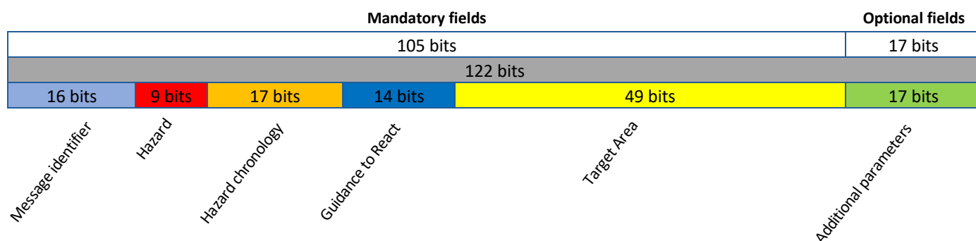
Figure 2: High Level Structure of CAMF
