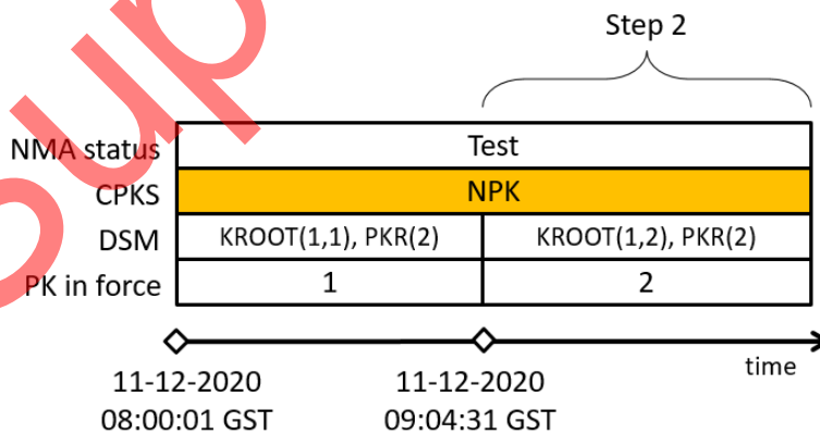
Figure 9: NPK Step 2 test vector
