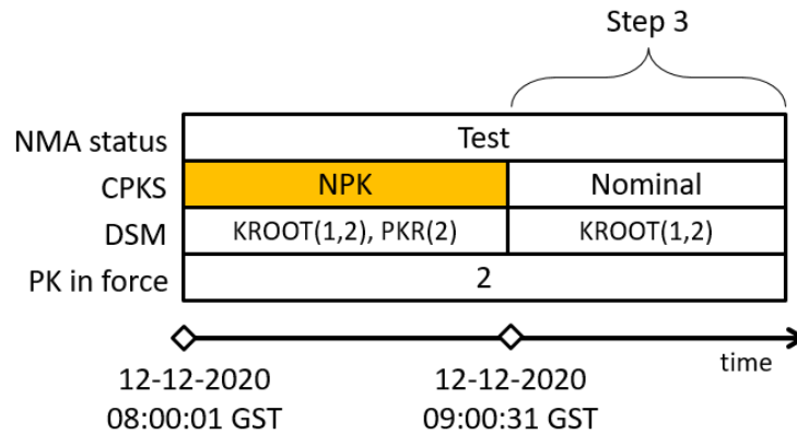
Figure 10: NPK Step 3 test vector
