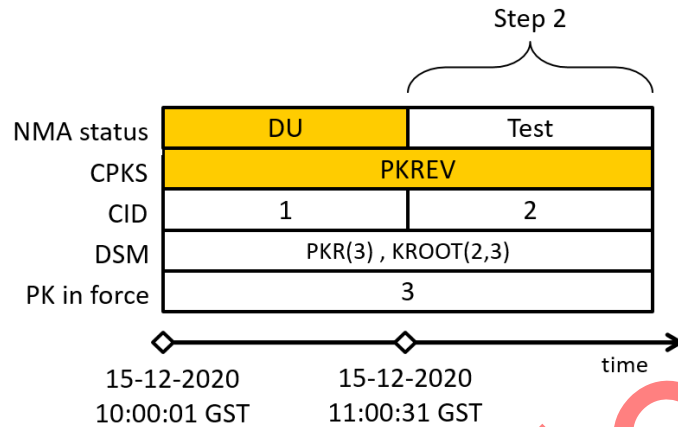
Figure 12: PKREV Step 2 test vector
